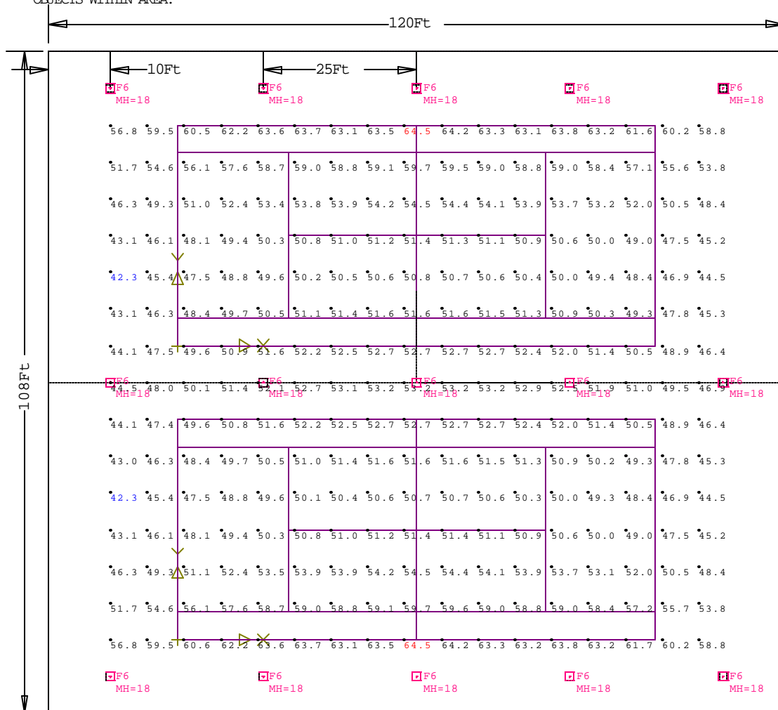
elevation view:Elevation Rotated-90 Tilted 90 Scale: 1 inch= 30 Ft.
