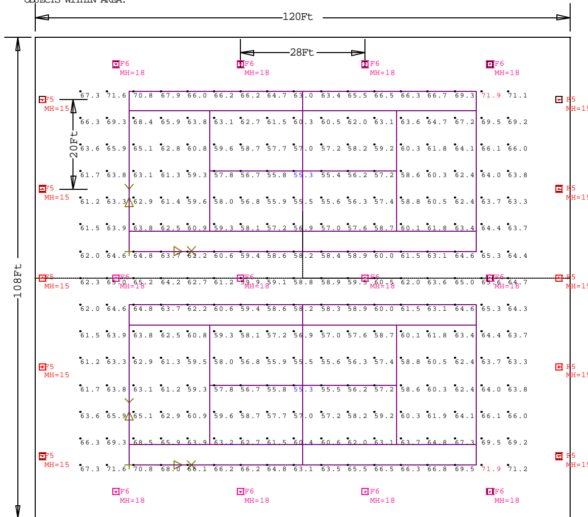
elevation view:Elevation Rotated-90 Tilted 90 Scale: 1 inch= 30 Ft.
